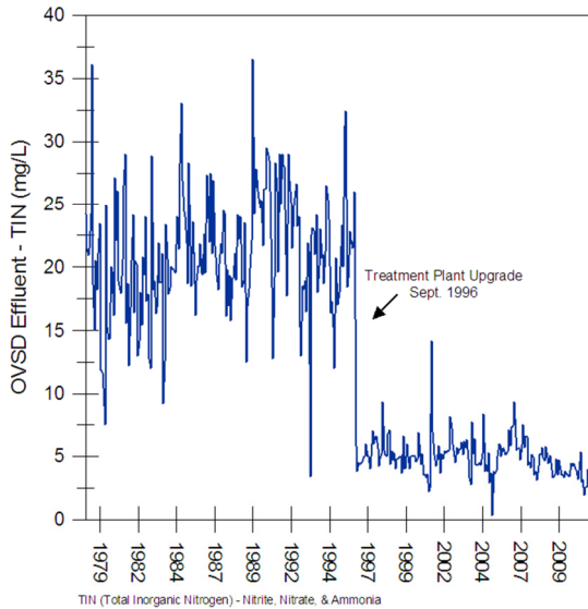
Figure 2-15 OVSD Effluent TIN Concentration 1979-2009
