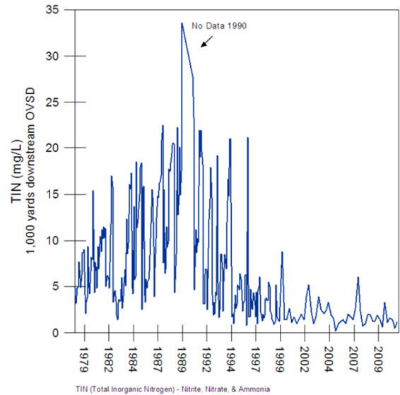
Figure 2-16 Ventura River TIN Concentration Downstream OVSD 1979-2009
