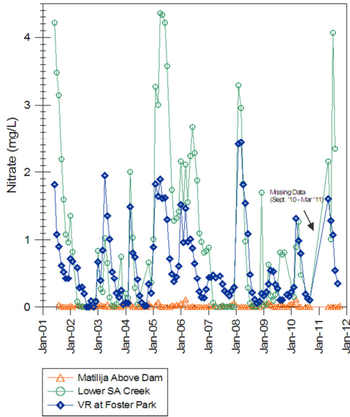
Figure 2-11 Nitrate Concentration Upper Watershed
