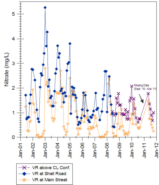
Figure 2-12 Nitrate Concentration lower watershed
