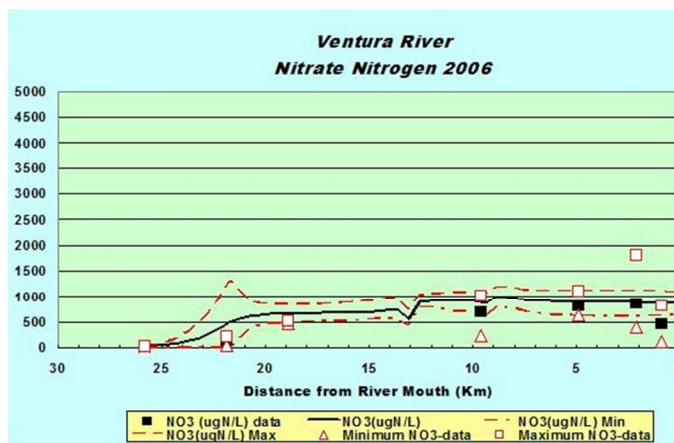
Figure 5-7 Comparison of calculated nitrate-nitrogen with 2006 observed data for validation
