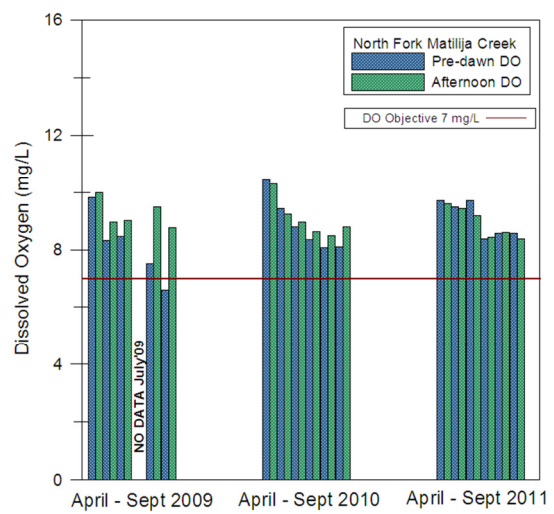
Figure 2-10 North Fork Matilija Creek DO Measurements
